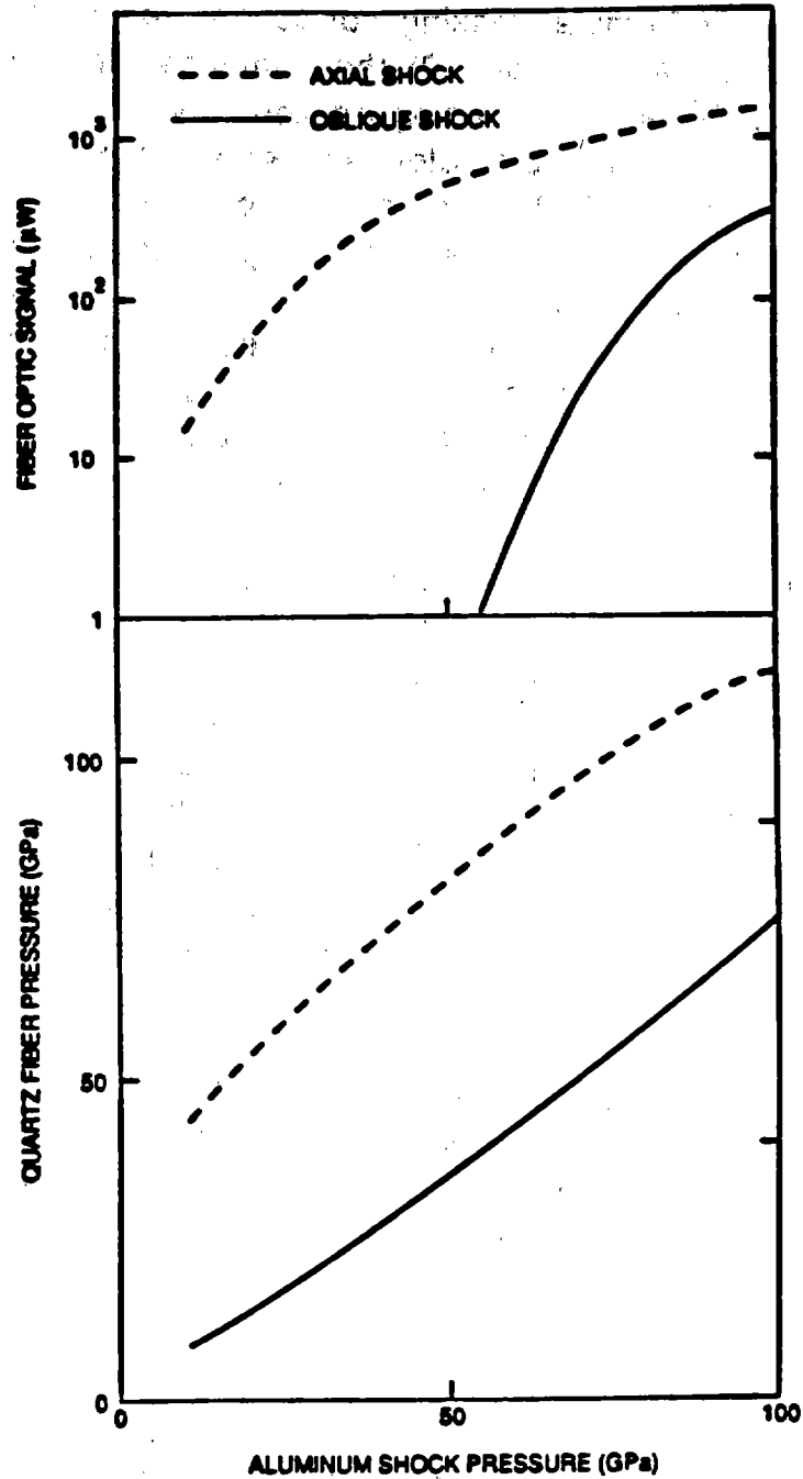
Figure 3. Calculated signals for 100- \mu\text{m} -diam-core optical fibers in shocked aluminum. A bandwidth of 300 nm around a central wavelength of 850 nm is assumed. When the shock runs along the fiber axis, the shock pressure is higher and more light is produced than for a shock oblique to the axis.
