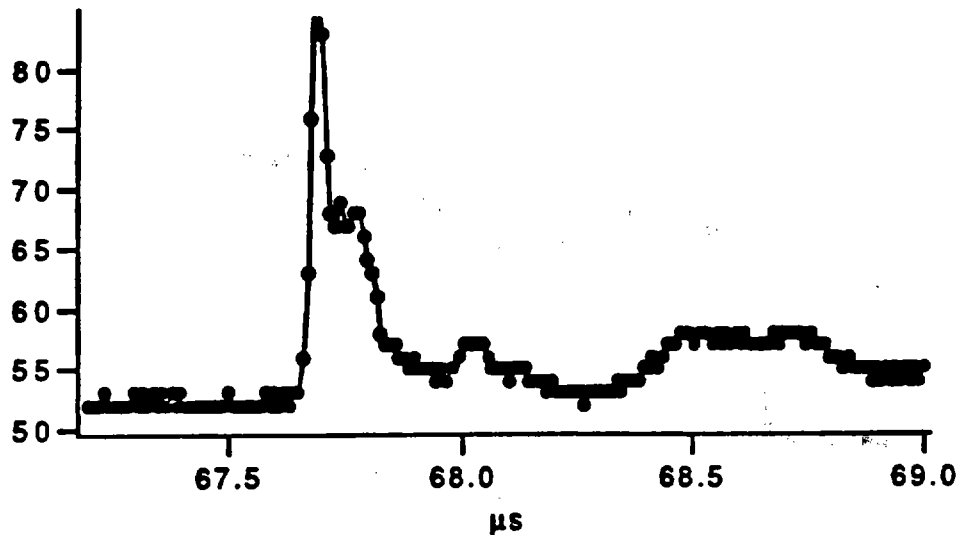
Figure 1. Data from an optical pin in contact with detonating high explosive. The vertical scale is roughly exponential with a peak value of a few hundred microwatts and a noise level of about 0.1 \mu W.
